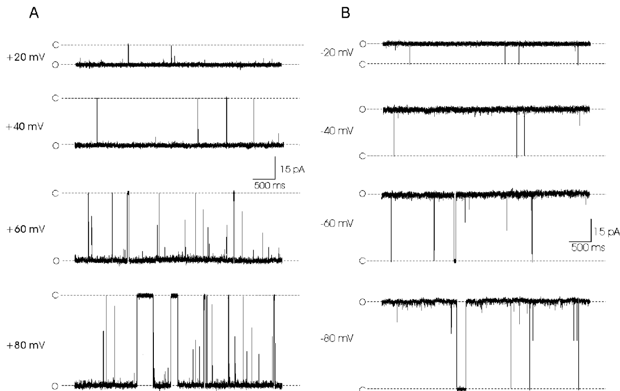
FIGURE 6 Voltage-dependent gating of the DIDS-modified RyR channel in symmetrical 210 mM KCl solutions. ( A ) and ( B ) illustrate current fluctuations through the channel at positive and negative holding potentials, respectively. Dotted lines labeled “O” and “C” indicate the fully open and fully closed levels, respectively. For clarity, examples of voltage-dependent inactivation events are not shown, but are illustrated in a separate figure (Fig. 9).
