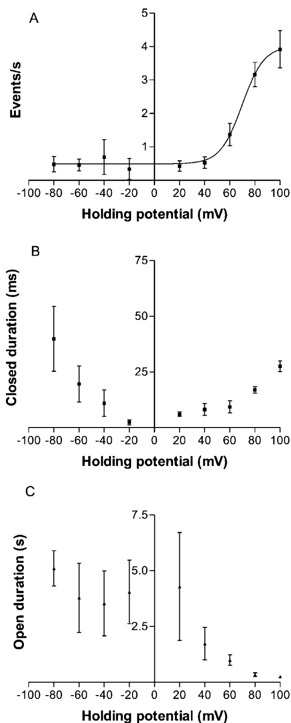
FIGURE 8 Voltage-dependence of the frequency ( A ), mean dwell times of the brief closing events ( B ), and the mean dwell times of the open events ( C ) of DIDS-modified channels. The solid line in ( A ) represents the Boltzmann distribution (fitted using GraphPad Prism (GraphPad Software Inc., San Diego, CA)) according to the equation y = (A_1 - A_2) / \{1 + \exp[(x - x_0)/dx]\} + A_2 , where A_1 and A_2 are the initial and final values respectively, x_0 is the voltage at which half the maximum effect was observed, and dx is the slope. dx is equivalent to RT/zF , where R is the universal gas constant, T is the temperature in K, F is the Faraday constant and z is the valence of the particle moving across the voltage drop. At 23°C RT/F = 25.5 ; z is therefore 25.6/ dx . This yielded a z value of 2.84. The mean values and SEM ( n = 4 ) are shown.
